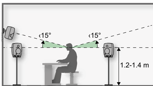
Monitor height (ITU-R BS.775-2 Recommendation)
